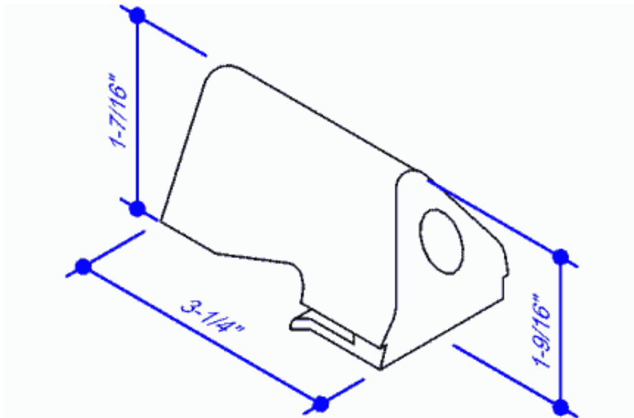
MR-24 Lockseam Plug
