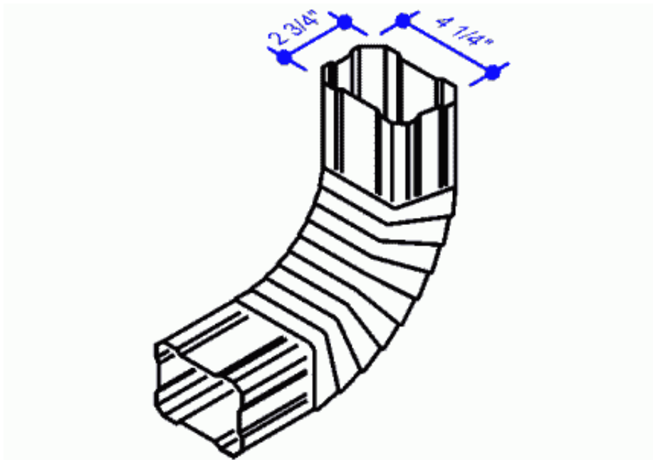
4" Conductor Elbow, 90 Degrees
