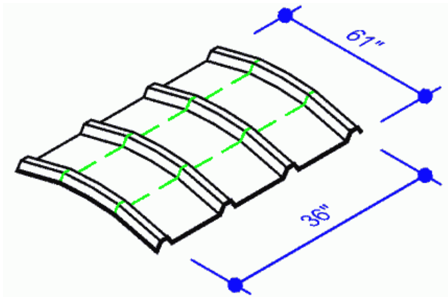
Butlerib Ridge Panel, 1:12 Slope
